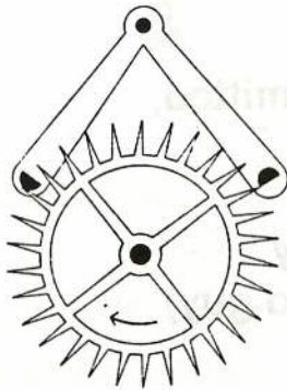
BROCOT PIN PALLET ESCAPEMENT
