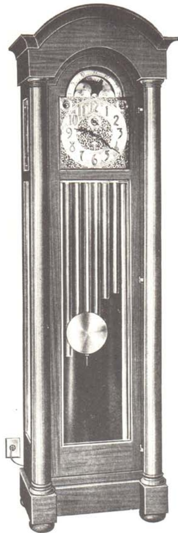
No. 86 Height, 92 inches Width, 25 inches Depth, 16 inches Colonial
